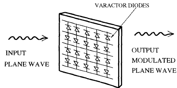
Fig. 1. Varactor diode analog grid modulator.
