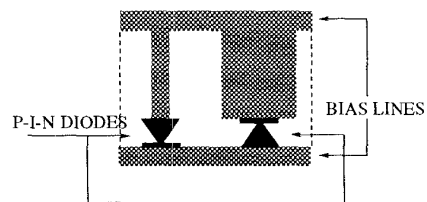
Fig. 2. Quasi-optical transmission-type BPSK grid modulator.
