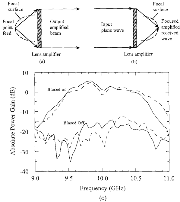
Fig. 2. The lens amplifier operating in (a) transmit mode and (b) receive mode. (c) Measured power gain and isolation of the quasi-optical lens amplifier used as a transmit lens (dashed lines) and receive lens (solid lines).
