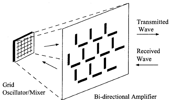
Fig. 1. A quasi-optical tranceive module consisting of a bi-directional amplifier and a grid oscillator/mixer.
