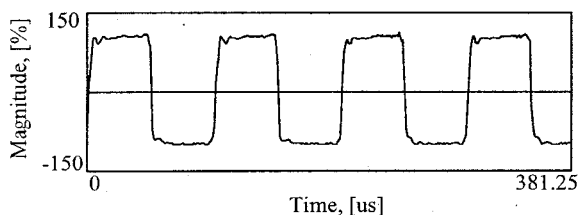
Fig. 8. AM demodulated 10 kHz squarewave signal received by a quasi-optical receiver front-end. The signal was AM modulated on a 10.1 GHz carrier, mixed to a 290 MHz IF frequency and demodulated using a vector signal analyzer.
