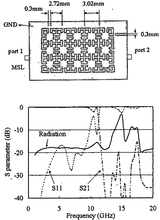
Fig. 5. Geometry of ground plane for the microstrip PBG described in [5] (top), along with simulated s-parameters and radiated power (bottom).
