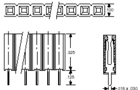
Female pin strip socket
