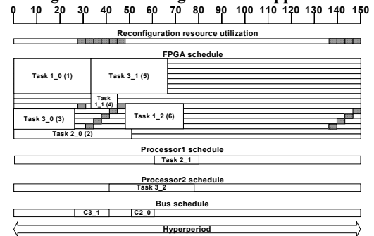
Figure 7: Scheduling result for Approach II
