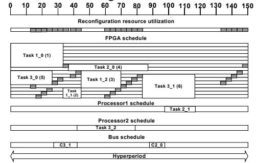
Figure 6: Scheduling result for Approach I
