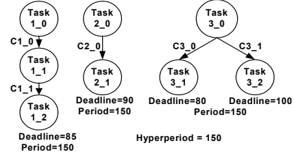
Figure 5: Task graphs
