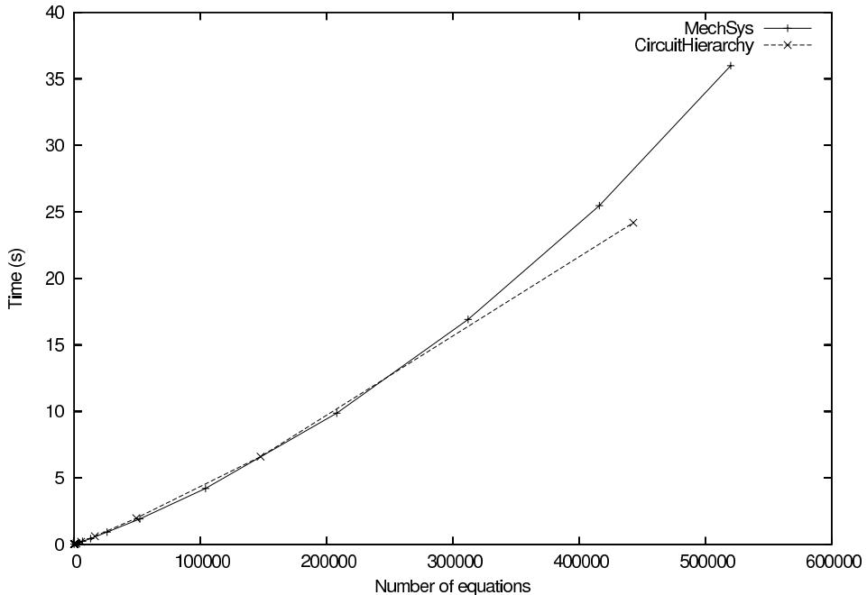
Figure 12.2: Elaboration time in relation to the number of generated equations.
