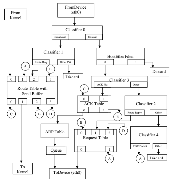
Figure 11: The Click DSR router
