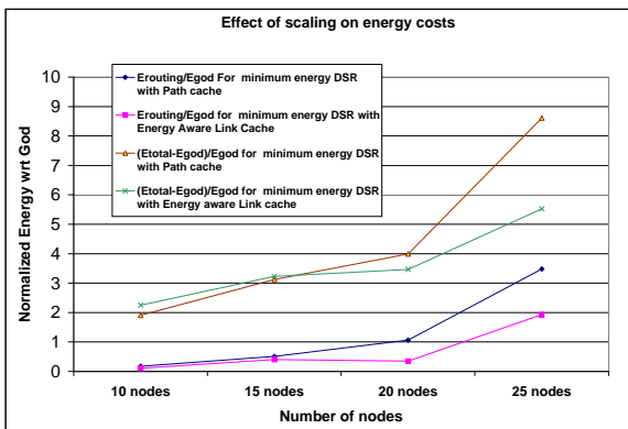
Figure 9: Effect of scaling on energy cost- Node speed 1 m/sec
