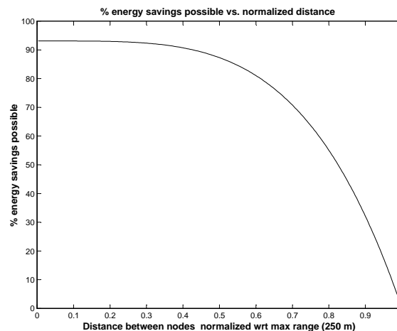
Figure 1: Energy savings possible using transmit power control
