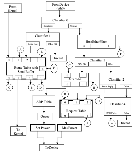
Figure 13: Energy Aware DSR implementation in Click
